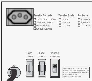
PAINEL TRASEIRO
